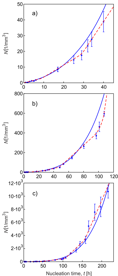
FIG. 4. Crystal number density vs nucleation time at 693 K. Rhombuses are the experimental data. The solid blue line was plotted by Eq. (9) with \zeta(t) approximated by the Kohlrausch stretched exponent equation [Eq. (8)]. The dashed red line corresponds to the stepwise evolution of the structural order parameter that allows the best description of the experimental data. Indexes correspond to different nucleation times considered in this analysis: short (a), average (b), and long (c) observations.
