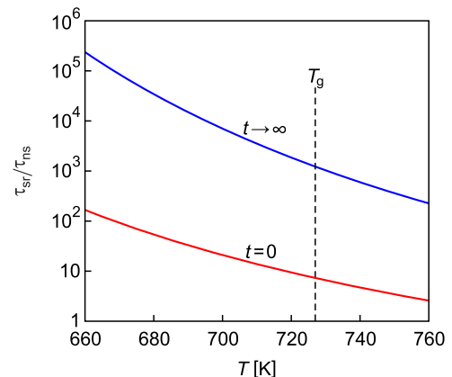
FIG. 10. The \tau_{sr}/\tau_{ns} time ratio as a function of temperature at the very beginning of the nucleation process ( t = 0 ) and at an advanced stage ( t \rightarrow \infty ).
