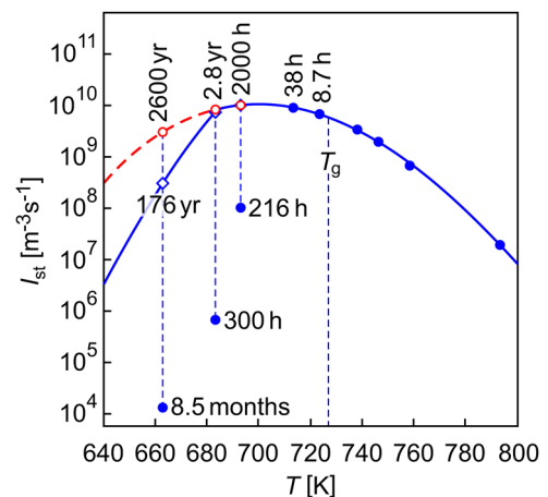
FIG. 9. Nucleation rates as a function of temperature. The dashed red line shows the theoretically expected nucleation rates, and the times \tau_{0.9} are denoted above the hollow circles. The solid blue line corresponds to the maximum nucleation rates that can be reached before significant crystallization, whereas the times \tau_{cr} are denoted close to the symbols. The solid circles show the experimentally measured nucleation rates that have been reached by the treatment times indicated.
