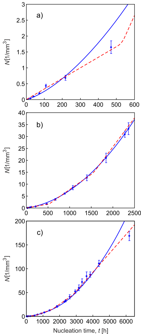
FIG. 2. Crystal number density vs nucleation time at 663 K. Rhombuses are the experimental data. The solid blue line was plotted by Eq. (9) with \zeta(t) approximated by the Kohlrausch stretched exponent equation [Eq. (8)]. The dashed red line corresponds to the stepwise evolution of the structural order parameter that allows the best description of the experimental data. Indexes correspond to different nucleation times considered in this analysis: short (a), average (b), and long (c) observations.
