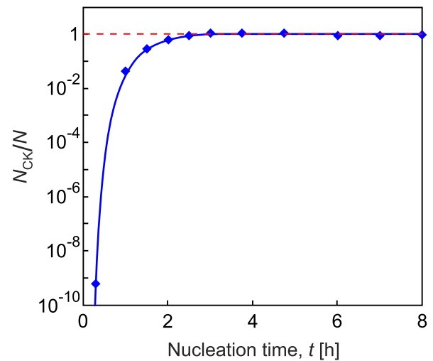
FIG. 7. N_{CK}/N ratio vs nucleation time at 723 K. Points denote the ratio of experimental values of N to those estimated by Eq. (10). The solid blue line was obtained as the ratio of N estimated by Eqs. (10) and (9). The dashed red line corresponds to the case when N is equal to N_{CK} .
