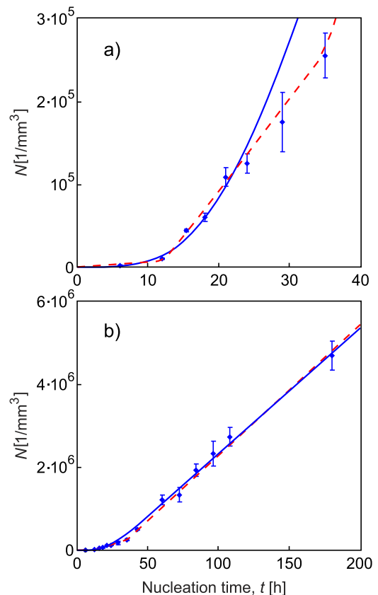
FIG. 5. Crystal number density vs nucleation time at 713 K. Rhombuses are the experimental data. The solid blue line was plotted by Eq. (9) with \zeta(t) approximated by the Kohlrausch stretched exponent equation [Eq. (8)]. The dashed red line corresponds to the stepwise evolution of the structural order parameter that allows the best description of the experimental data. Indexes correspond to different nucleation times considered in this analysis: short (a) and average (b) observations.
