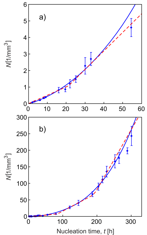
FIG. 3. Crystal number density vs nucleation time at 683 K. Rhombuses are the experimental data. The solid blue line was plotted by Eq. (9) with \zeta(t) approximated by the Kohlrausch stretched exponent equation [Eq. (8)]. The dashed red line corresponds to the stepwise evolution of the structural order parameter that allows the best description of the experimental data. Indexes correspond to different nucleation times considered in this analysis: short (a) and average (b) observations.
