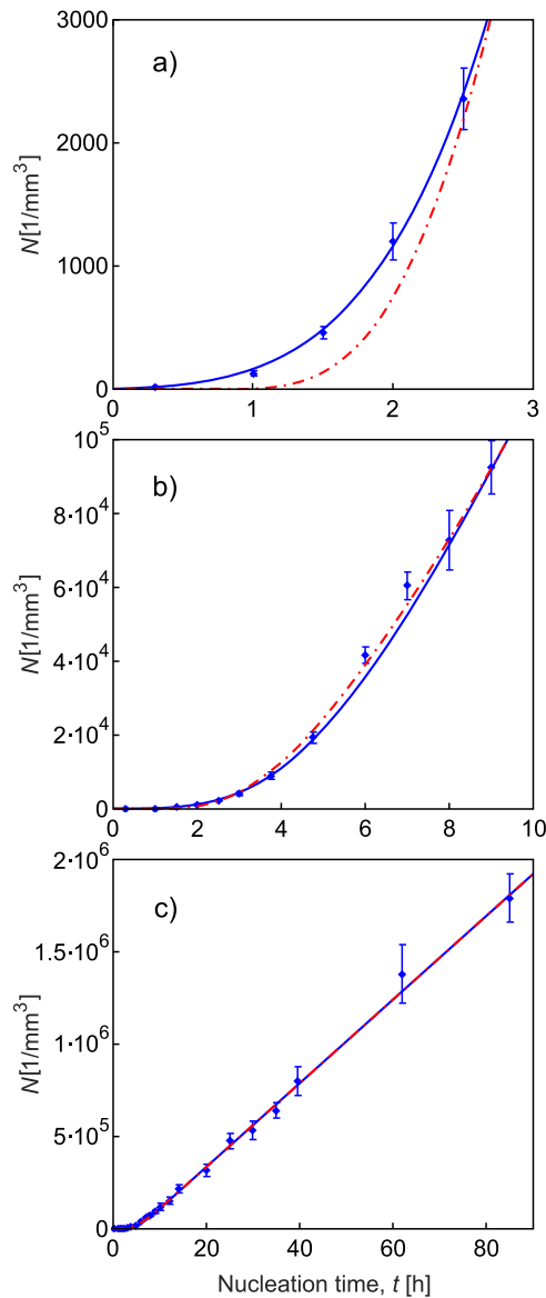
FIG. 6. Crystal number density vs nucleation time at 723 K. Rhombuses are the experimental data. The solid blue line was plotted by Eq. (9) with \zeta(t) approximated by the Kohlrausch stretched exponent equation [Eq. (8)]. The dashed-dotted red line corresponds to the Collins–Kashchiev equation [Eq. (10)] with I_{st} = 6.3 \times 10^9 \text{ m}^{-3} \text{ s}^{-1} determined by Eq. (1) at t \rightarrow \infty and \tau_{CK} = 3.2 \text{ h} used as a fit parameter to describe the linear part of the experimental N(t) –dependence. Indexes correspond to different nucleation times considered in this analysis: short (a), average (b), and long (c) observations.
