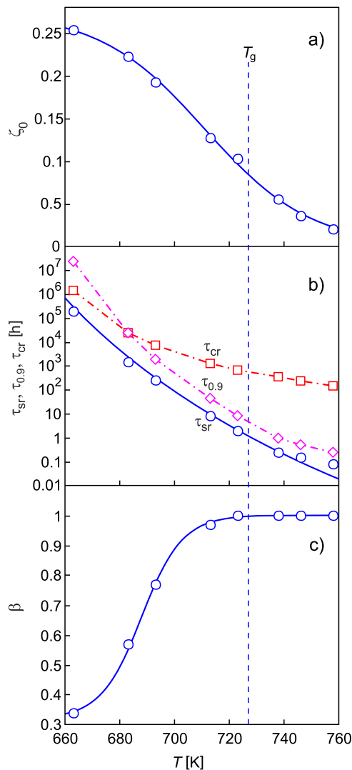
FIG. 8. Temperature dependences of the Kohlrausch stretched exponential parameters \zeta_0 , \tau_{sr} , and \beta (a, b, and c, respectively), as a function of temperature parameters; the times \tau_{0.9} and \tau_{cr} needed to achieve 0.9 I_{st}(T) and the volume fraction crystallized, \alpha = 0.99 , respectively. The solid blue lines are plotted by Eqs. (11)–(13), respectively. The dashed–dotted lines are only a guide to the eyes.
